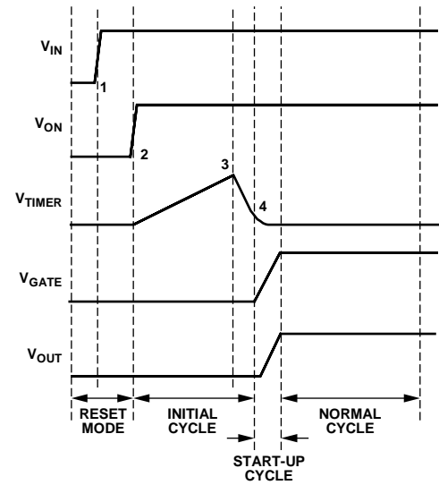
Figure 36. Power-Up Timing
